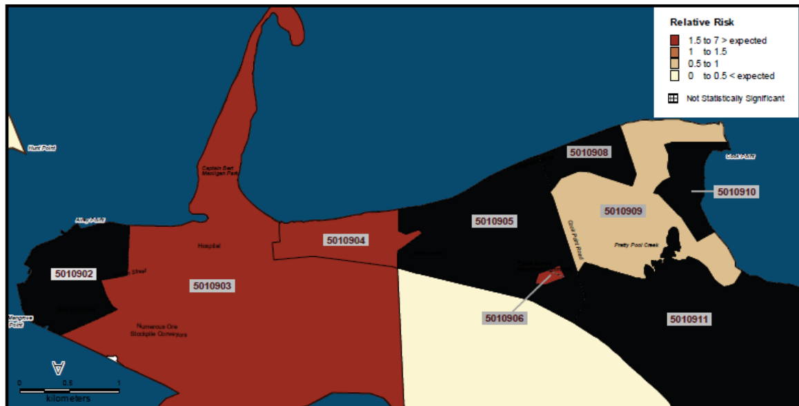
Figure 2: Map of Risk Estimates for Cardiovascular Hospital Admissions Port Hedland 1993-2004.
