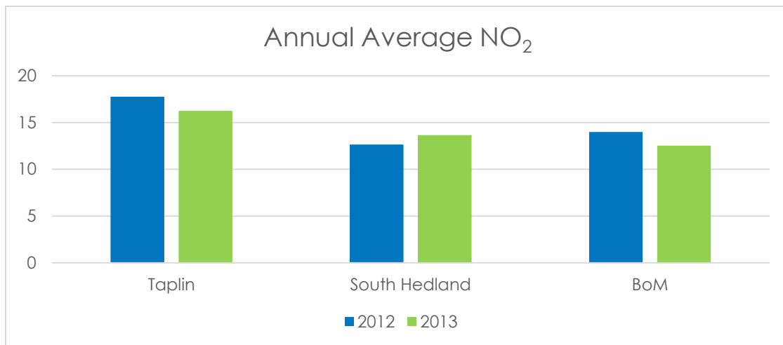
Figure 16: Annual Average NO 2 levels
