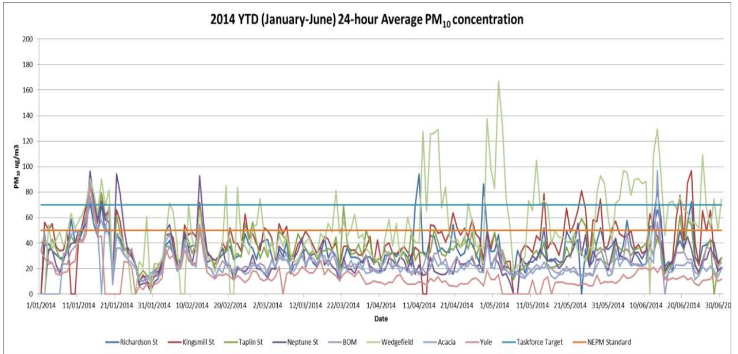
Figure 7: 2014 24-hour PM_{10} concentrations at all locations – January – June inclusive
