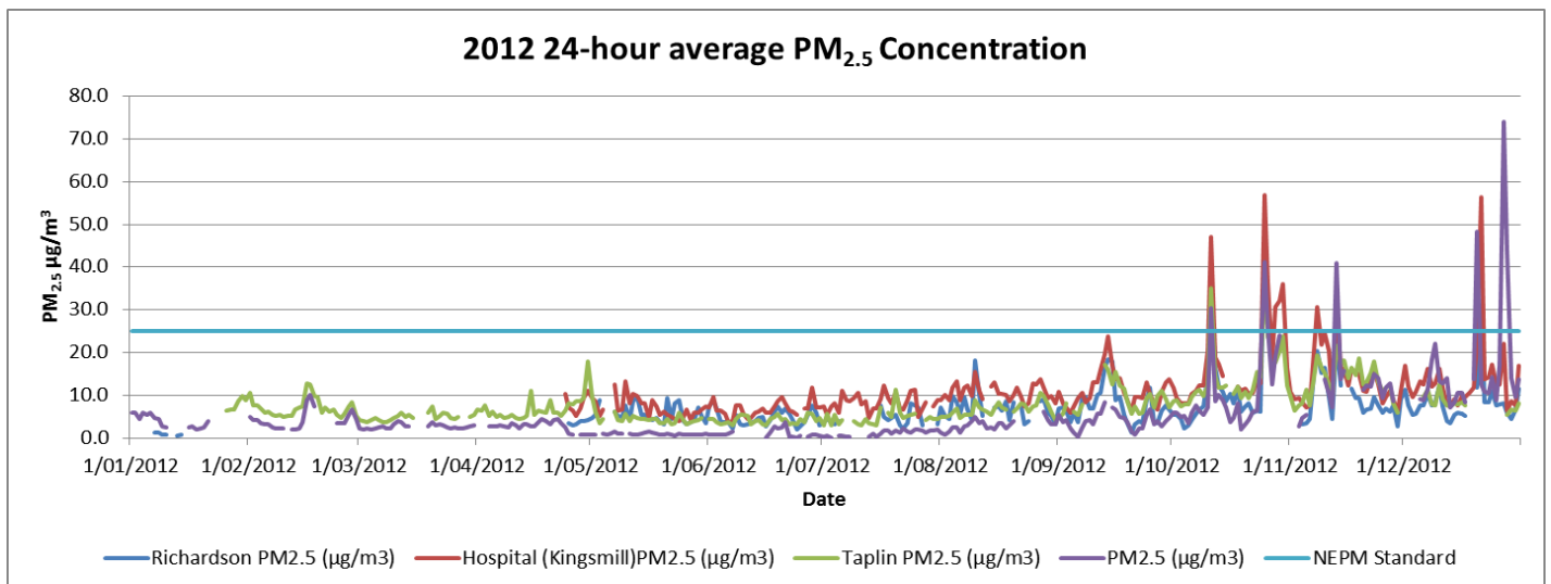
Figure 8: 2012 24-hour PM_{2.5} concentrations at all locations – shows exceedances of the NEPM standard for PM_{2.5} exclusively associated with bushfire days between October and December.
