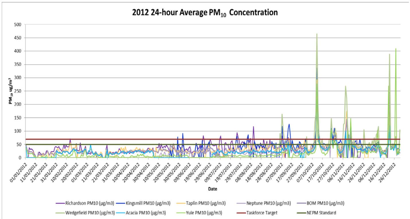
Figure 5: 2012 24-hour PM 10 concentrations at all locations (Wedgefield monitoring begins in October)
